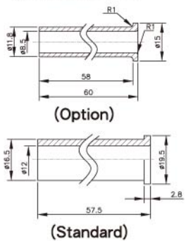
RUBBER TUBE FOR PLS-28-PM
