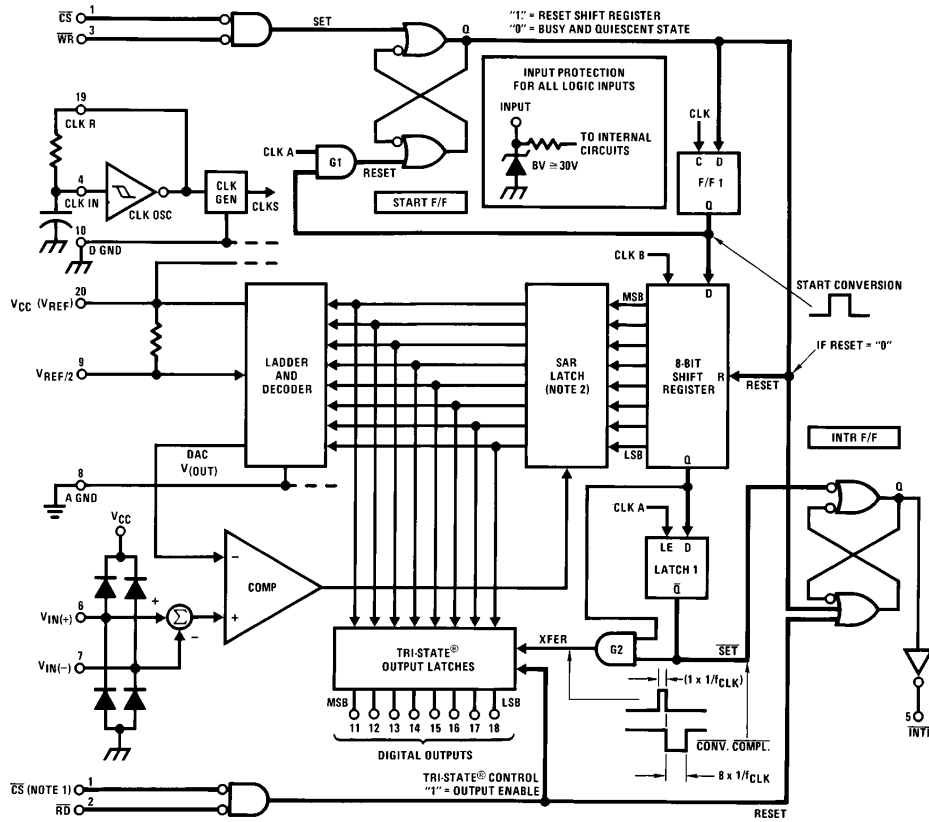
FIGURE 2. Block Diagram
