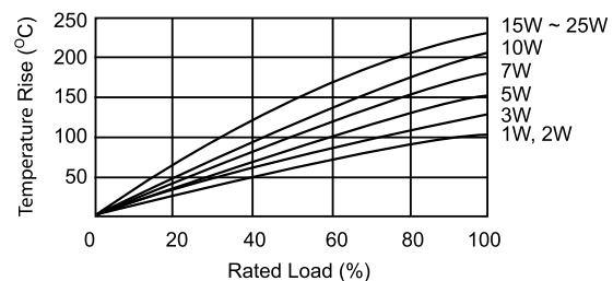
Heat Rise Chart
