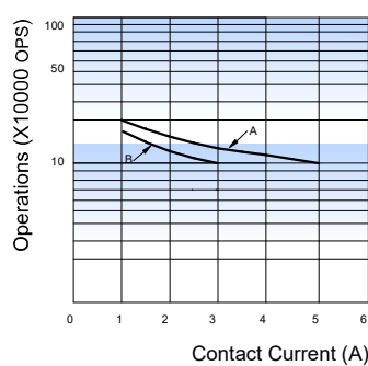
EDURANCE CURVE
