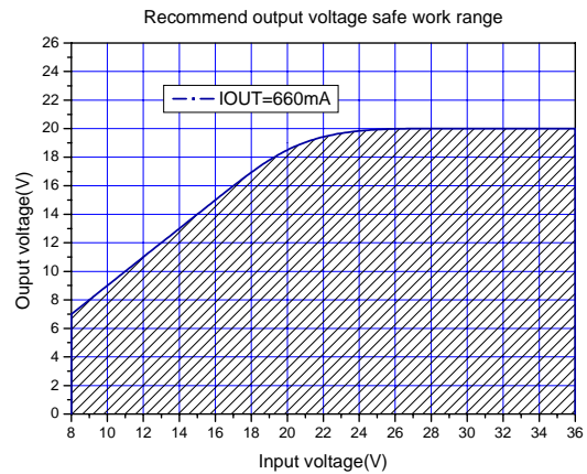
Figure13.Max output voltage(IOUT=660mA)
